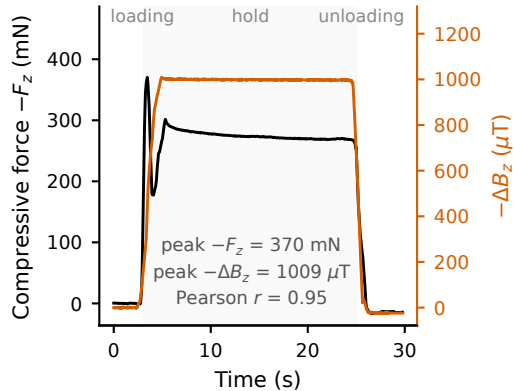
a Single load-hold-unload event
