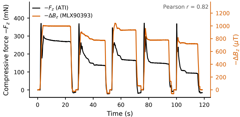
b Five consecutive load-unload cycles (manual loading)
