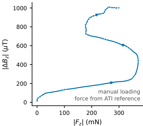
a Loading branch, single manual press
