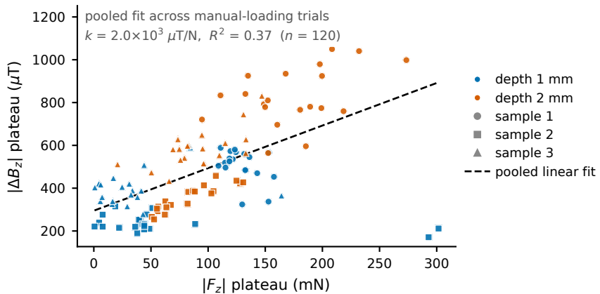
b Plateau amplitudes, manual-loading trials
