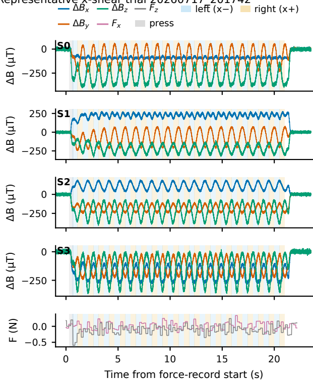
a Representative x-shear trial 20260717_201742
