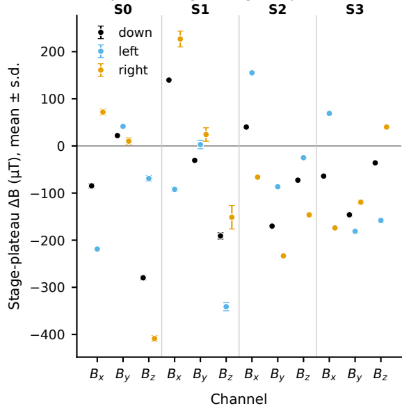
b Cycle-averaged stage response (18 trials)
