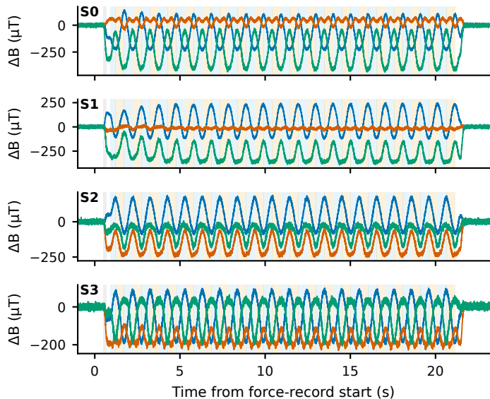
a Representative trial 20260717_204652
