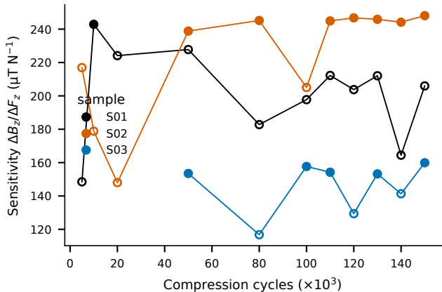
f4 150k-cycle durability (open = &gt;9% bad packets)
