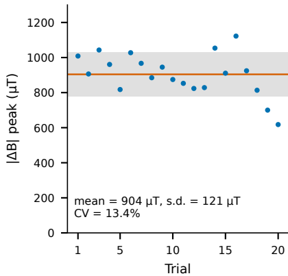
f3 Peak amplitude (manual taps)
