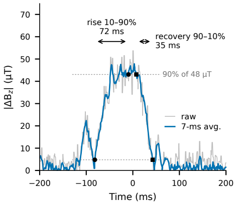
f1 Tap response event (manual loading)
