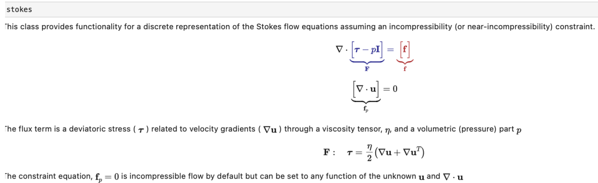
Figure 1: Underworld3 is integrated with Jupyter and with sympy. The development environment is easy to use, close to the original mathematical formulation and highly interactive. Once ready for deployment, parallel execution is efficient and scalable - no modification of the notebooks is needed.
