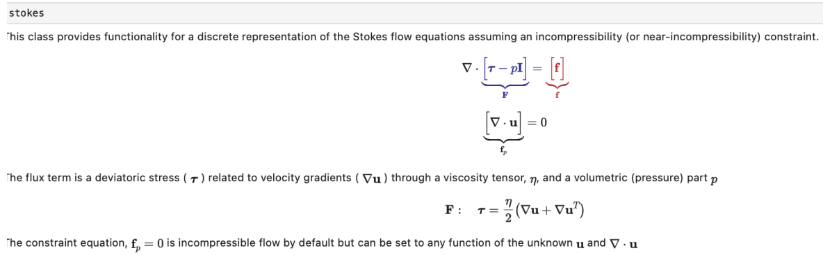
Figure 1: Underworld3 is integrated with Jupyter and with sympy. The development environment is easy to use, close to the original mathematical formulation and highly interactive. Once ready for deployment, parallel execution is efficient and scalable - no modification of the notebooks is needed.
