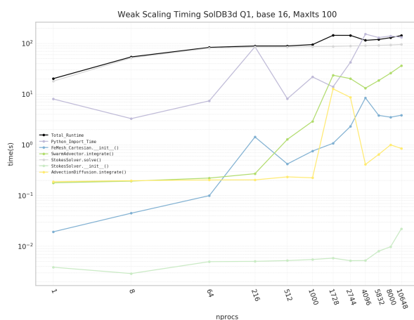
Figure 1: Gadi - v2.11-prerelease: Weak scaling of SolDB3D (linear elements) to \sim 10k procs
