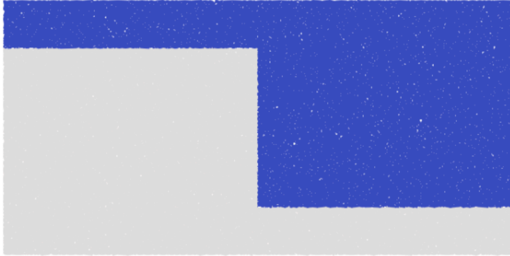
Fig.1 Model initial setups (128 km * 64 km).
