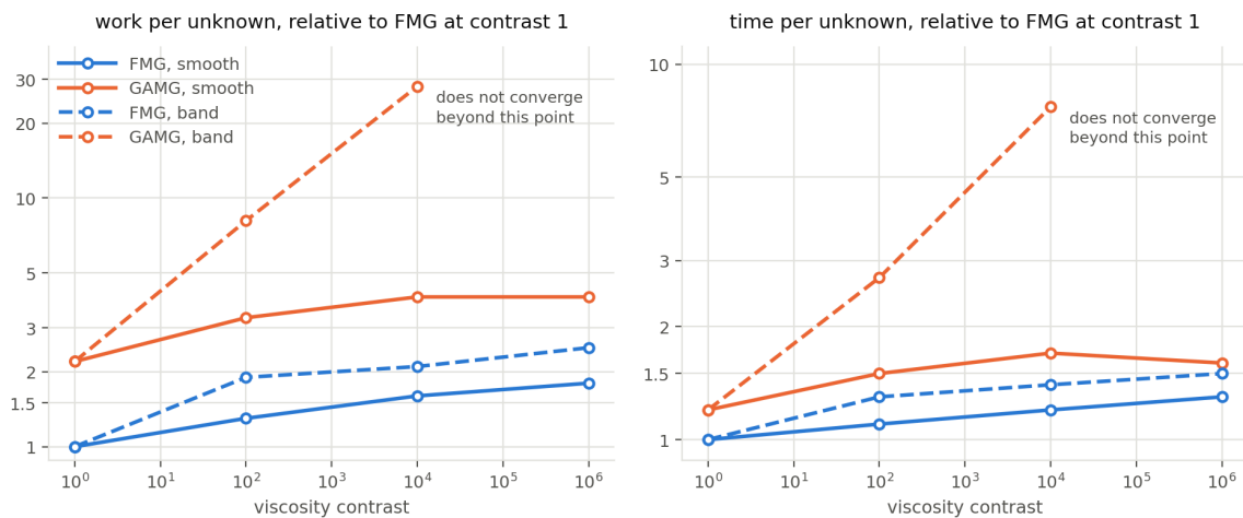
Figure 2: Cost against viscosity contrast for the two viscosity distributions, at 11 727 unknowns. FMG is almost indifferent to the change. GAMG is not: on the band its cost climbs with the contrast, and at 10^6 it does not converge at all — 20 000 multigrid cycles per velocity solve without reaching the tolerance. This is not an artefact of an under-resolved band. At this resolution the band spans about six cells, and resolving it better does not rescue GAMG: at four and sixteen times the cell count, GAMG's disadvantage against FMG on the band grows from 5.5 to 7.9 to 8.0 times its disadvantage on the smooth problem at the same size.
