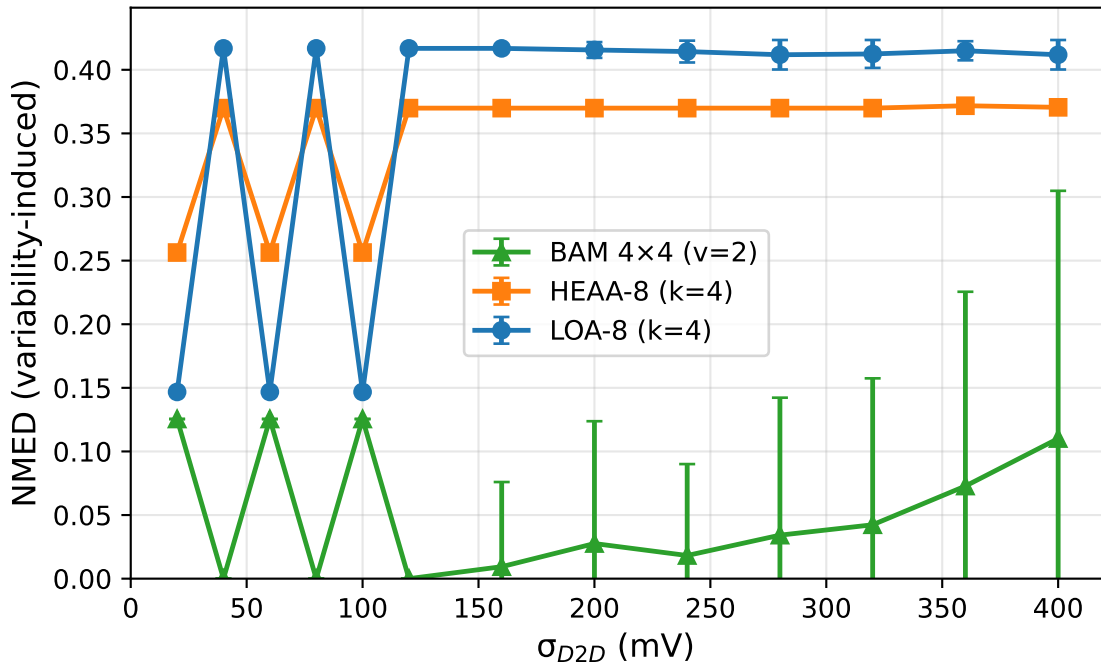
FeFET Variability Impact on CiM Outputs
