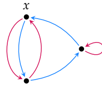
FIGURE 5.2: Alternative representation of the \underline{O}(S^1 \vee S^1) -set X from Figure 5.1, using colors and arrows to represent which parts lie over which circle in which orientation.
