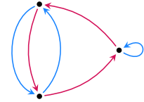
FIGURE 4.8: An “abnormal” bicycle with only the identity symmetry.
