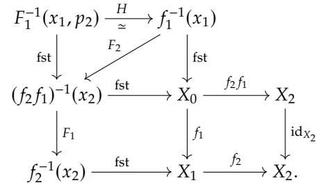
FIGURE 9.2: Crossing horizontal and vertical fiber sequences.
