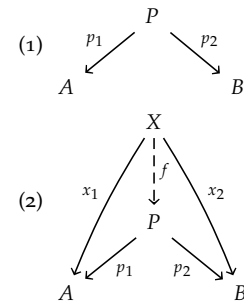
FIGURE 6.3: (1) A product cone, and (2) its universal property.
