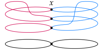
FIGURE 5.1: An \underline{O}(S^1 \vee S^1) -set X for which \text{ev}_x is not surjective. At the bottom the type S^1 \vee S^1 is visualized as two circles with a common base point. Note that the underlying set of X with the red and the blue permutation is a bicycle in the sense of Definition 4.6.1.
