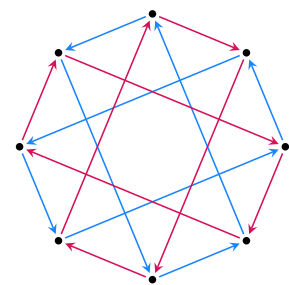
FIGURE 4.6: The quaternion bicycle.
