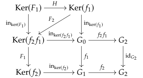
FIGURE 9.3: Kernels of composite homomorphisms.
