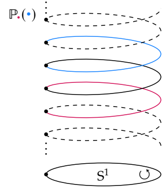
FIGURE 3.5: For the fiber of the universal set bundle, \mathbb{P}_{\bullet}(\bullet) \equiv (\bullet \rightrightarrows \bullet) , we increase the winding number when we transport the endpoint (in blue) along \cup , and we decrease it when we transport the starting point (in red) in the same way.
