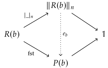
FIGURE 3.15: Taking summands for b:B in Figure 3.14.
