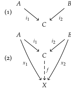
FIGURE 6.4: (1) A coproduct cocone, and (2) its universal property.
