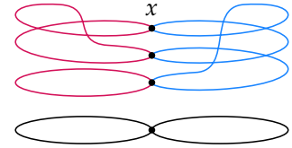
FIGURE 5.1: An \underline{O}(S^1 \vee S^1) -set X for which \text{ev}_x is not surjective. At the bottom the type S^1 \vee S^1 is visualized as two circles with a common base point. Note that the underlying set of X with the red and the blue permutation is a bicycle in the sense of Definition 4.6.1.
