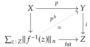
FIGURE 9.4: Two n -Image factorizations of f .
