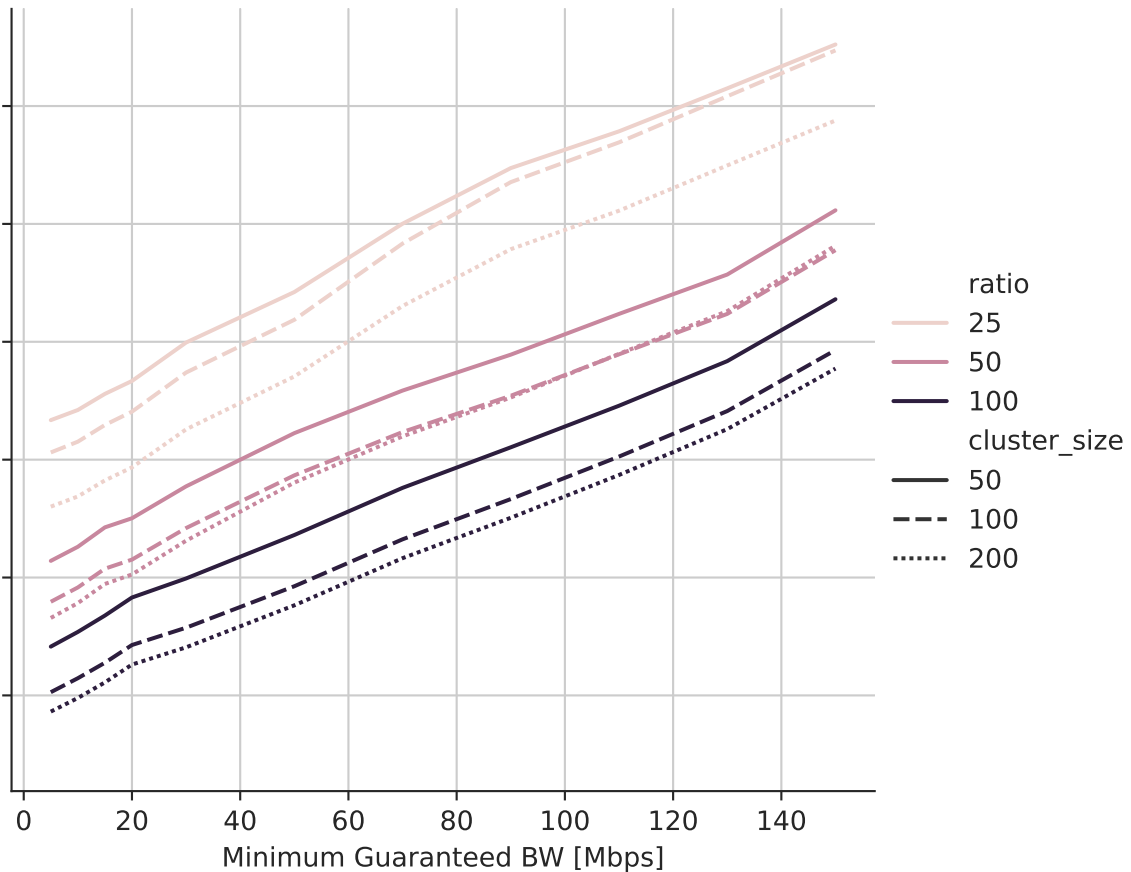
device = 802.11ad_pro
