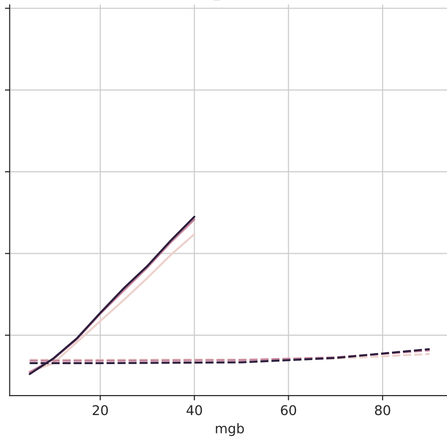
cluster_size = 100
