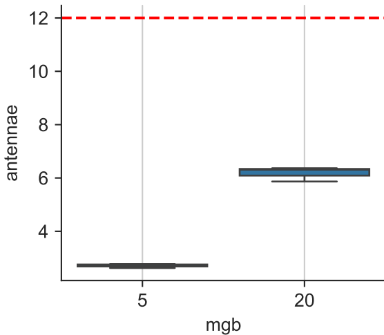
device = 802.11ac
