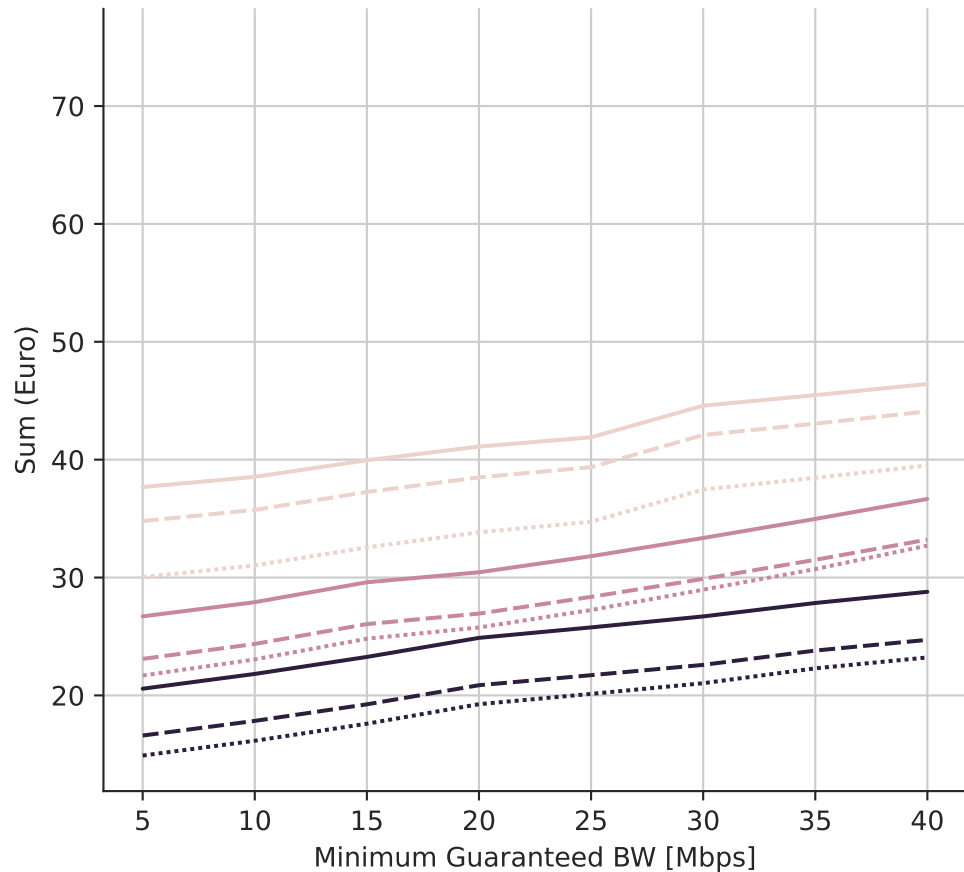
device = 802.11ac
