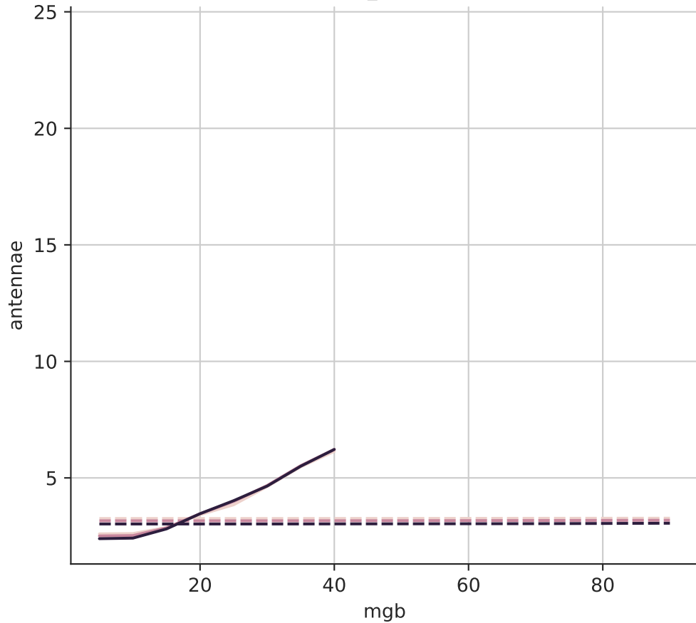
cluster_size = 50
