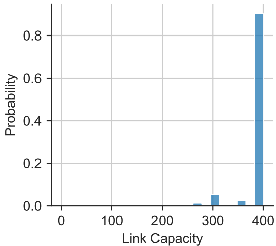
technology = 802.11ac
