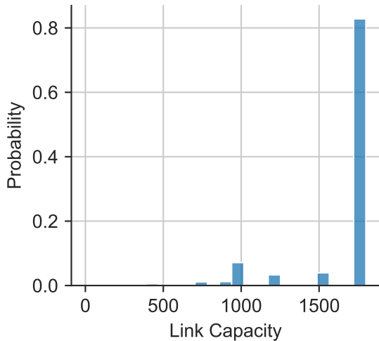
technology = 802.11ad_pro
