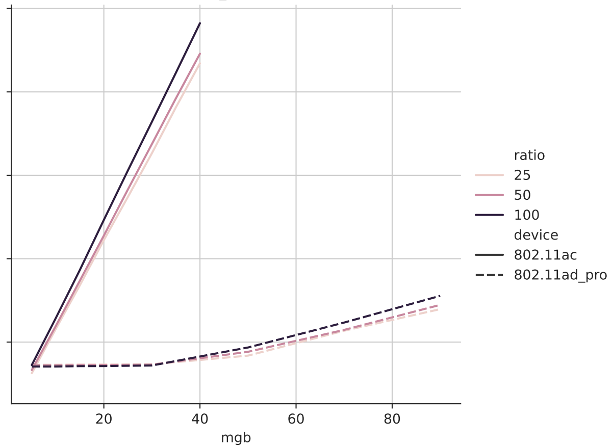
cluster_size = 200
