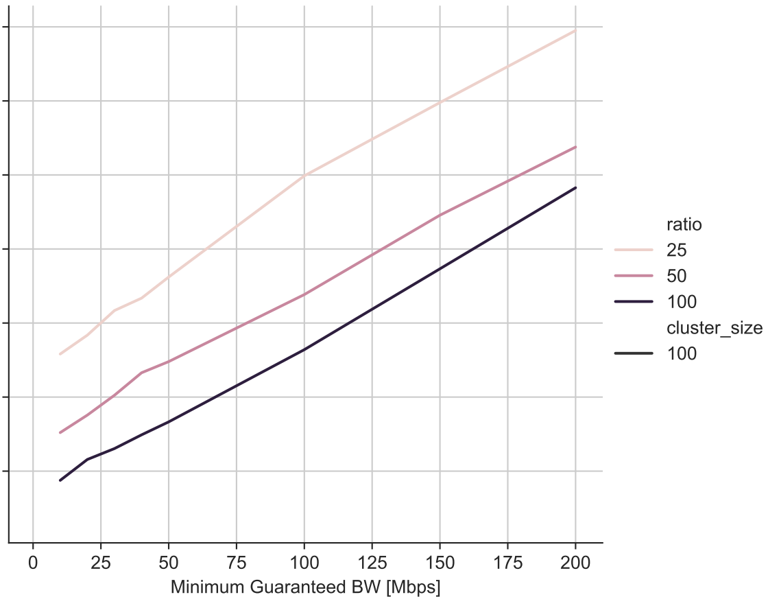
device = 802.11ad_pro
