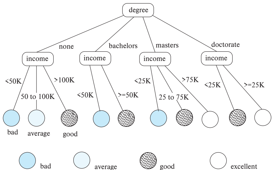
Figure 11.11 Classification tree.
