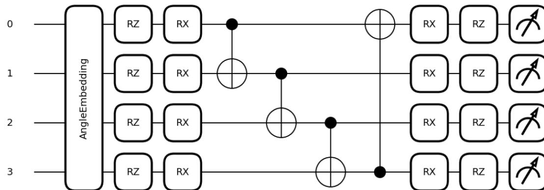
deep: n=4 qubits, L=4 layers (64 quantum parameters) one variational layer drawn; it is applied 4× between AngleEmbedding and measurement
