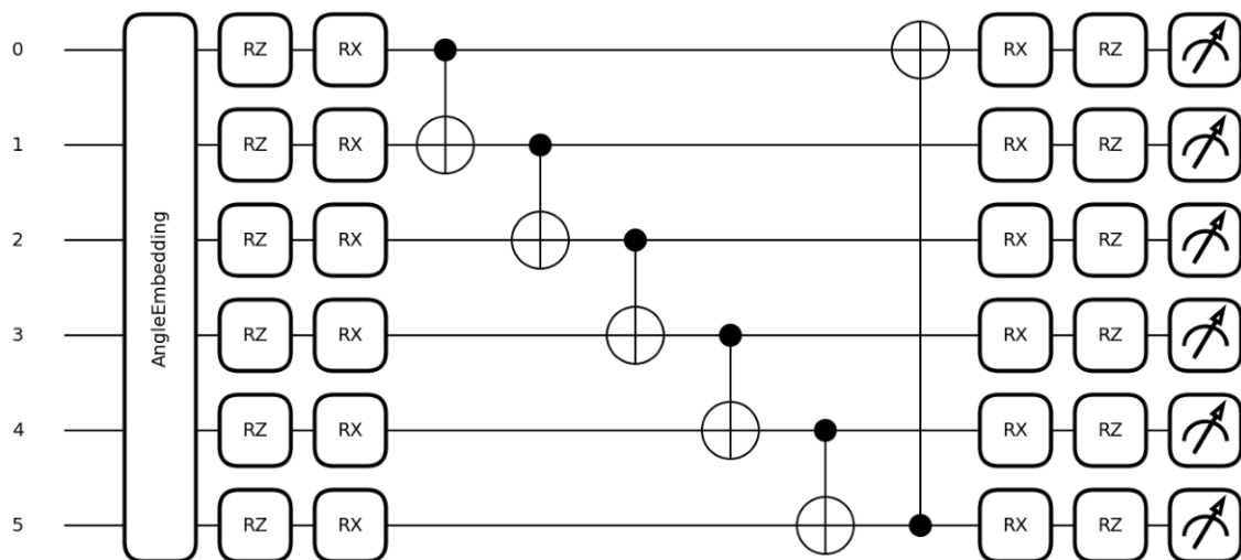
wide: n=6 qubits, L=2 layers (48 quantum parameters) one variational layer drawn; it is applied 2× between AngleEmbedding and measurement
