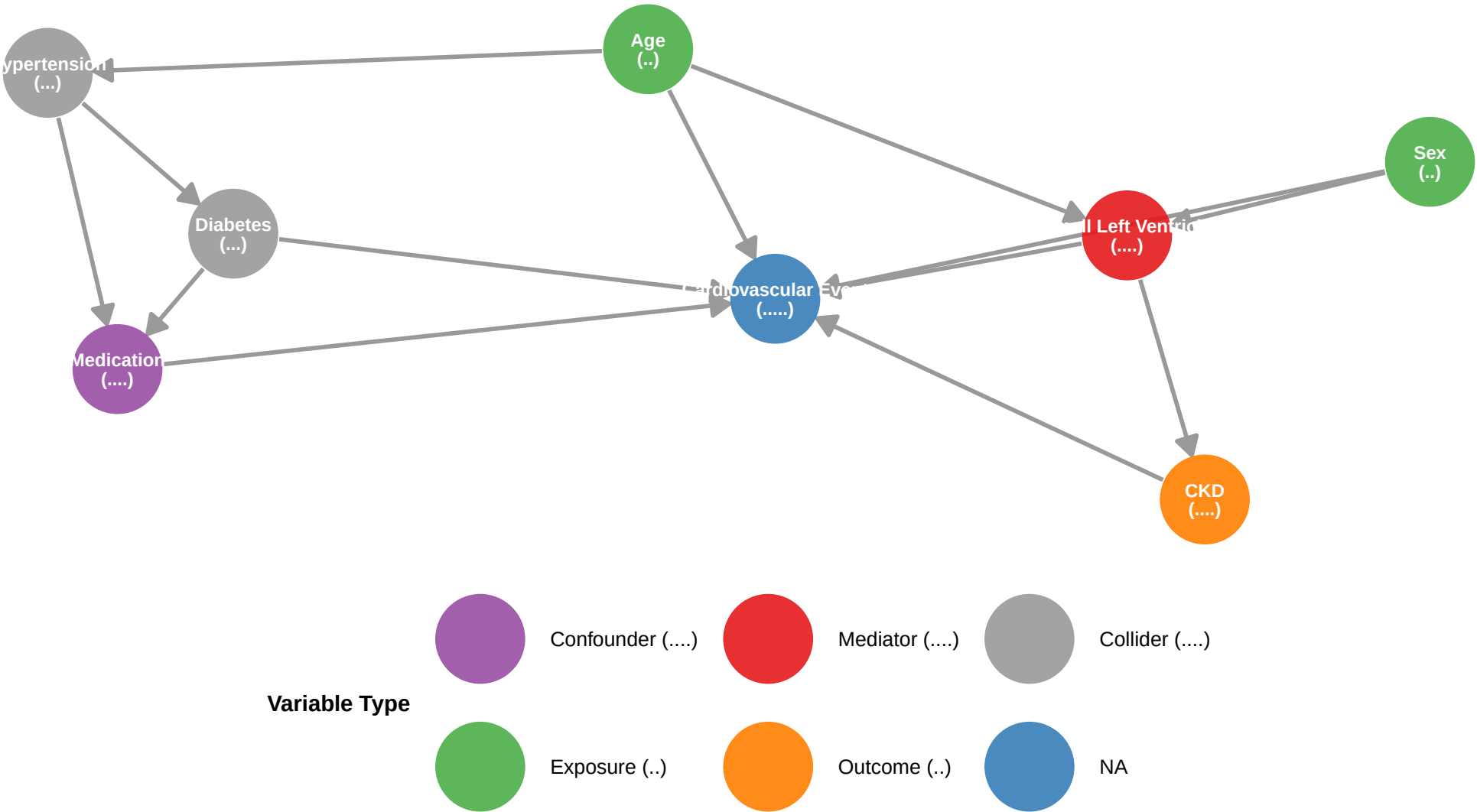
Figure 1. Directed Acyclic Graph (DAG) for Causal Relationships
