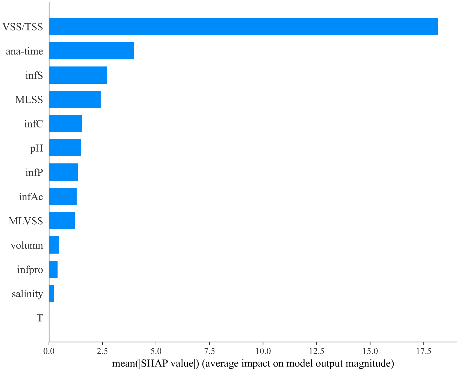
SHAP_numpy Sorted Feature Importance
