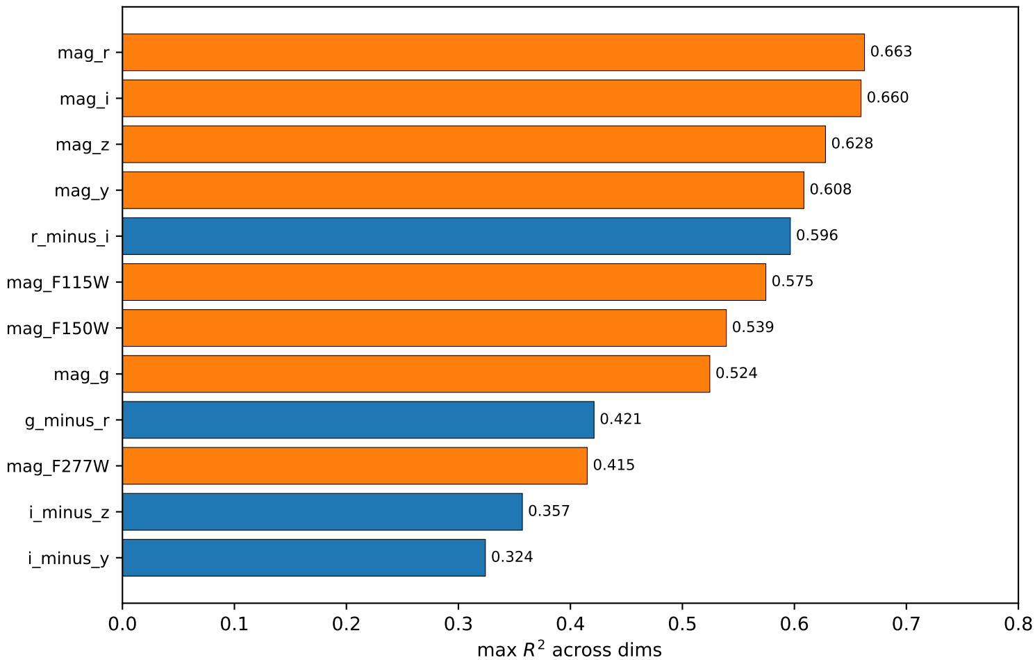
HSC — top covariates by max R^2
