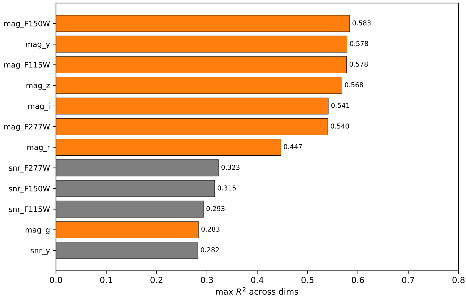
JWST — top covariates by max R^2
