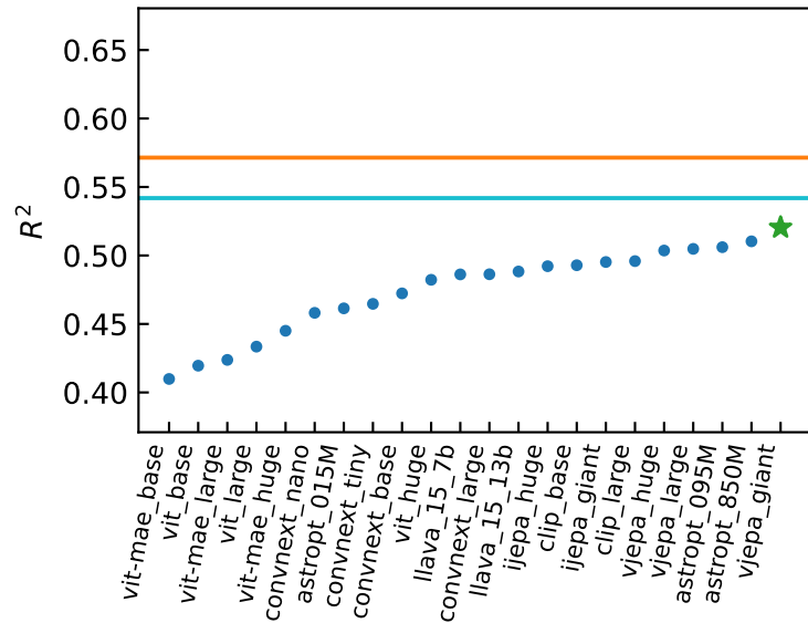
HSC
