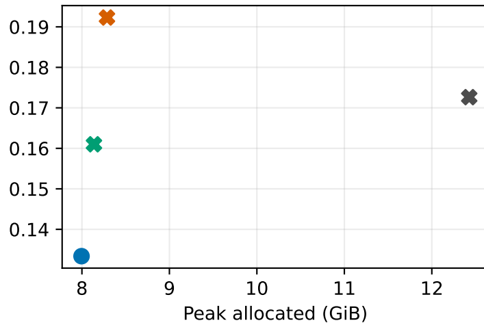
KITTI
