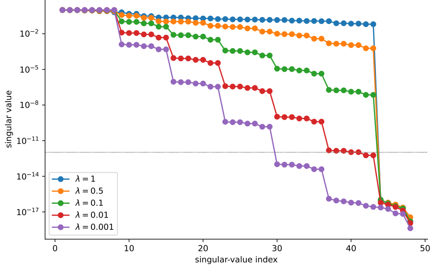
Fig. 2: Singular values of the saturated observation matrix \mathcal{O}_{r-1} for P = 8 , r = 6 , and L = r - 1 = 5 . Unlike Figure 1, this figure does not plot rank versus horizon. The horizon is fixed, and the horizontal axis is the singular-value index i = 1, \dots, 48 . Each curve shows the singular values s_i(\mathcal{O}_{r-1}) in decreasing order for one value of \lambda . The exact saturated rank is 43, so five singular values are zero in exact arithmetic. The effective rank reported in Table 1 is obtained by counting how many singular values lie above the declared tolerance. For small \lambda , some algebraically nonzero singular values fall below this tolerance, which explains the effective-rank loss seen in Figure 1. The dotted horizontal line marks the corresponding SVD tolerance; for these parameters the tolerance levels nearly coincide across \lambda .
