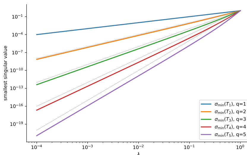
Fig. 3: Conditioning of the collar-to-queue map T_q from Theorem 2. Each solid curve shows \sigma_{\min}(T_q) as a function of \lambda for q = 1, \dots, 5 . The dotted reference curves show \lambda^q . The deepest exposed collar coordinate enters the queue with a factor of order \lambda^q , so exact recovery becomes ill-conditioned when \lambda is small. This explains why exact observability and floating-point effective observability can differ.
