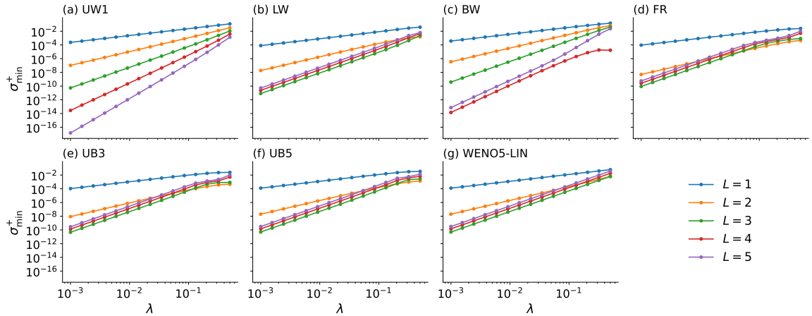
Fig. 3: E3: smallest nonzero singular value of the single-parent observation map versus Courant number (log–log), one panel per scheme, horizons L = 1, \dots, 5 . Slopes match the predicted exponents \gamma = L_q of conjecture 2 (table 4). Panels (left to right, top to bottom): (a) UW1, first-order upwind; (b) LW, Lax–Wendroff; (c) BW, Beam–Warming; (d) FR, Fromm; (e) UB3, upwind-biased p = 3 ; (f) UB5, upwind-biased p = 5 ; (g) WENO5-LIN, linear-weights WENO5 (+FE).
