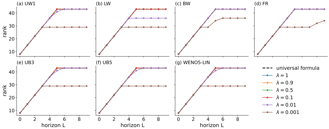
Fig. 1: Rank ladders for the linear scheme family: effective (SVD) rank of \mathcal{O}_L versus horizon L for P = 8 , r = 6 , one panel per scheme, six Courant numbers, overlaid with the universal formula P + (P - 1) \min\{L, r - 1\} (black dashed). For \lambda \geq 0.1 , every curve coincides with the dashed universal ladder for every scheme, confirming theorem 1; departures at \lambda \leq 0.01 are effective-rank (conditioning) losses, not violations of the theorem. Panels (left to right, top to bottom): (a) UW1, first-order upwind; (b) LW, Lax-Wendroff; (c) BW, Beam-Warming; (d) FR, Fromm; (e) UB3, upwind-biased p = 3 ; (f) UB5, upwind-biased p = 5 ; (g) WENO5-LIN, linear-weights WENO5 (+FE).
