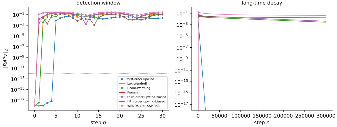
Fig. 6: E5: coarse separation \|R(A_\lambda^{[\text{sch}]})^n v\|_2 of the deepest sharp pair per scheme. Left: detection window — each curve sits at the roundoff floor ( \sim 10^{-17} ) through step t_0 - 1 and crosses the threshold (dotted) exactly at the predicted step, t_0 = 5 for UW1 down to t_0 \leq 1 for the widest stencils. Right: long-time decay over 3 \times 10^5 steps — the detection ordering reverses; first-order upwind erases its trace almost immediately on this axis while the high-order schemes retain theirs for 10^5 – 10^7 steps (table 5).
