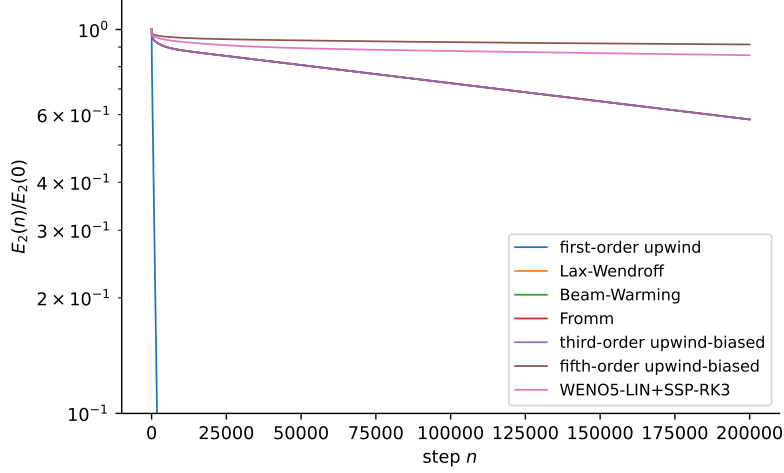
Fig. 5: E4d: step-function flattening — norm retention E_2(n)/E_2(0) , with E_2(n) the \ell^2 norm of the zero-mean (nonconstant) part of the state after n steps — over 2 \times 10^5 steps ( N = 64 , \lambda = 0.5 ). The vertical axis is clipped at 10^{-1} so that the high-order members can be compared; first-order upwind exits the frame by step n \approx 2 \times 10^3 and continues geometrically—a straight line on the logarithmic axis with per-step factor \rho_N = 0.99880 —reaching 10^{-17} by n \approx 3.2 \times 10^4 , in agreement with the slowest-mode prediction \ln(10^{17})/(-\ln \rho_N) \approx 3.25 \times 10^4 . Every high-order member still retains 58%–91% of its nonconstant L^2 norm at the end of the run. Only four of the seven curves are distinguishable: at \lambda = \frac{1}{2} LW/BW and FR/UB3 coincide pairwise — exactly — and the two pairs differ by less than the line width (remark 14(iii)).
