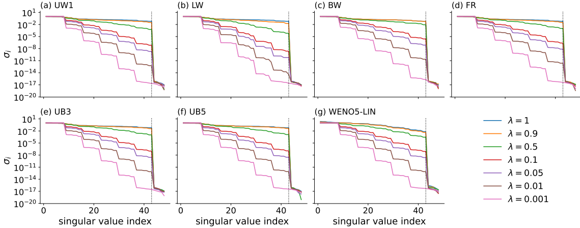
Fig. 2: Singular spectra of the saturated observation matrix \mathcal{O}_{r-1} ( P = 8, r = 6 ), one panel per scheme, seven Courant numbers. The dotted vertical line marks the exact rank 43. Spectra to the right of steep drops fall below the declared tolerance and are lost to effective rank; Lax–Wendroff’s class- m=4 node degeneracy is visible as the early plateau collapse at \lambda = 0.01 . Panels (left to right, top to bottom): (a) UW1, first-order upwind; (b) LW, Lax–Wendroff; (c) BW, Beam–Warming; (d) FR, Fromm; (e) UB3, upwind-biased p = 3 ; (f) UB5, upwind-biased p = 5 ; (g) WENO5-LIN, linear-weights WENO5 (+FE).
