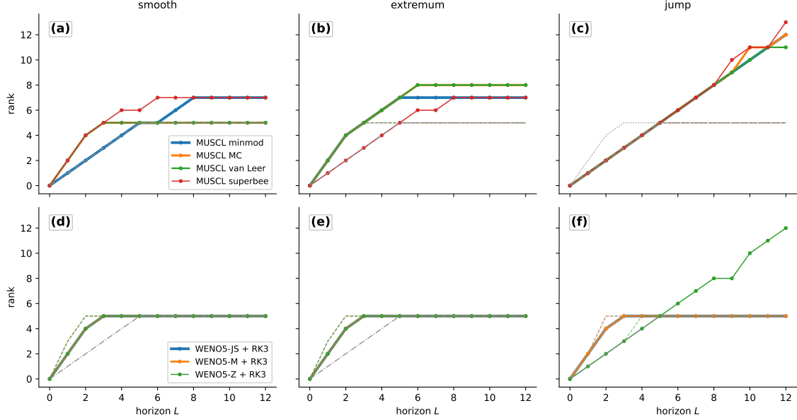
Fig. 7: E6: empirical response-span (solid, \varepsilon = 10^{-5} , floor \theta = 10^{-3} ) and linearized (dashed) local ladders in the three base-state regimes, for the MUSCL family (top row) and the WENO5 family (bottom row): (a) MUSCL, smooth; (b) MUSCL, extremum; (c) MUSCL, jump; (d) WENO5, smooth; (e) WENO5, extremum; (f) WENO5, jump. Gray references (Jacobian-response baselines): the two-collar law \min(2L, r-1) (dotted) and the one-collar law \min(L, r-1) (dash-dotted). Smooth regime: minmod follows \sigma = 1 , the other limiters \sigma = 2 ; at the extremum, the minmod and superbee roles swap. Jump regime: all MUSCL linearizations collapse to UW1 ( \sigma = 1 ), while the response-span ladders continue past the linear budget r-1 = 5 at one direction per step. In panels (d) and (e), the three WENO5 variants coincide exactly and are drawn with nested line widths so each stays visible; the mechanism and its significance are discussed in section 7.6 .
