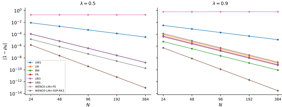
Fig. 4: E4c: |1 - \rho_N| versus N (log-log) at \lambda = 0.5 (left) and 0.9 (right). Slopes match the dissipative orders -2s of proposition 6 to three decimals; the flat top curve is the WENO5-LIN + FE instability ( \rho_N > 1 , N -independent). At \lambda = 0.5 the four 2s = 4 semi-Lagrangian members overlay: LW/BW and FR/UB3 coincide pairwise exactly at this \lambda , and the two pairs share the leading coefficient A = \frac{3}{64} ( remark 14(iii) ).
