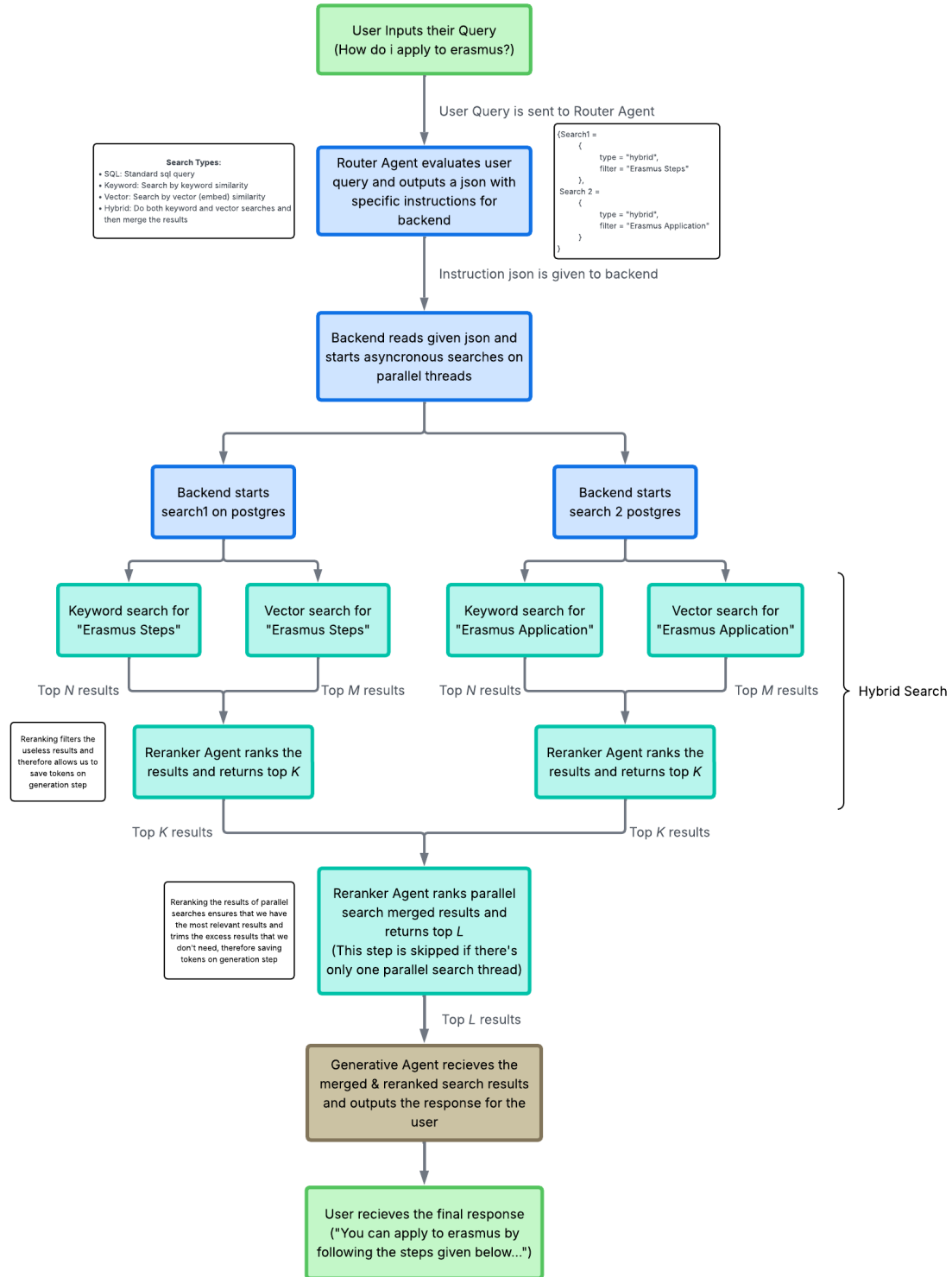
Figure 4: End-to-end RAG chatbot pipeline. The Router Agent converts the user query to a structured intent list; the backend dispatches parallel hybrid searches; each search undergoes Reranker-scored ranking before results are merged, optionally re-ranked across intents, and passed to the Generative Agent for a streamed final response.
