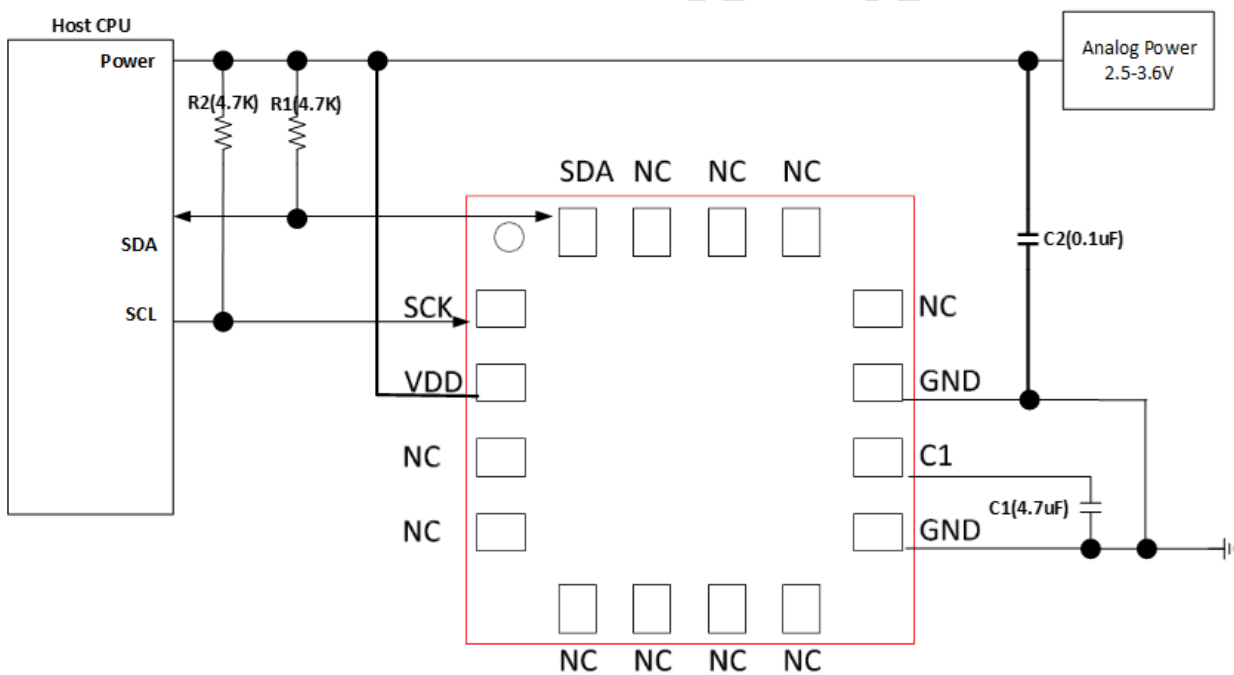
Figure 6. External Connection
