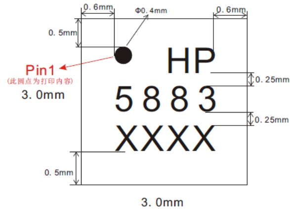
Figure 5. Chip Marking
