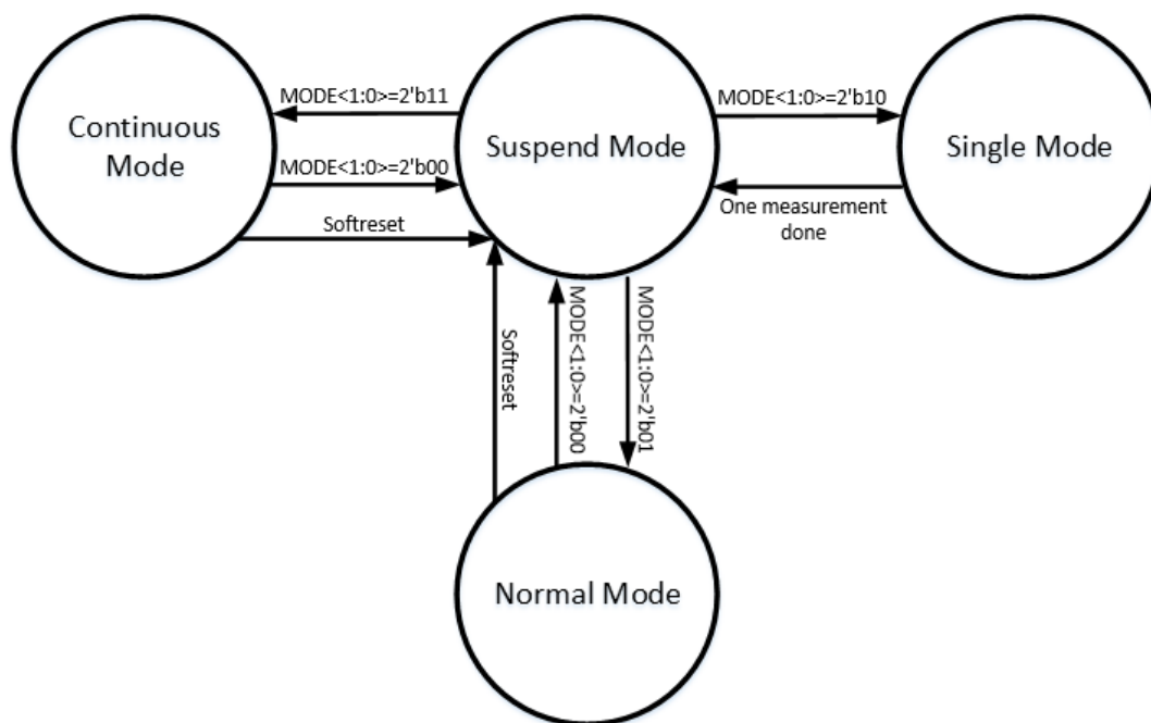
Figure 9. Modes Transition
