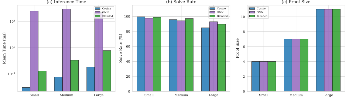
Fig. 11. GNN-ATSS vs. Cosine-ATSS vs. Blended-ATSS on 50 random provable formulas. All three configurations achieve identical proof quality (size 3–11, depth 1–7); runtime differences reflect per-inference overhead of GNN message-passing vs. O(1) cosine lookup.
