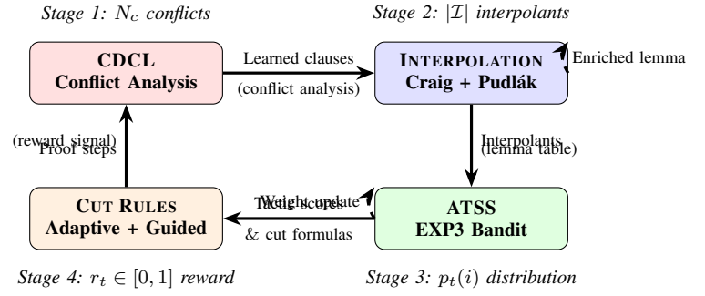
Fig. 2: The NEUROPROOF Virtuous Cycle. Stage 1: CDCL conflict analysis produces N_c learned clauses per refutation. Stage 2: Incremental Craig interpolation extracts |Z| interpolants, populating the global lemma table. Stage 3: ATSS maintains an exponential-weight distribution p_t(i) over 11 tactics; interpolant-stored lemmas bias the weight toward LEMMA_LEARN and INTERPOLATION_GUIDED_CUT. Stage 4: Successful proof derivations produce reward r_t , which updates ATSS weights via importance-weighted estimates (Equation (15)), closing the loop. Dashed arcs indicate self-reinforcement: richer interpolants enable better lemma reuse, and higher weights sharpen tactic selection.
