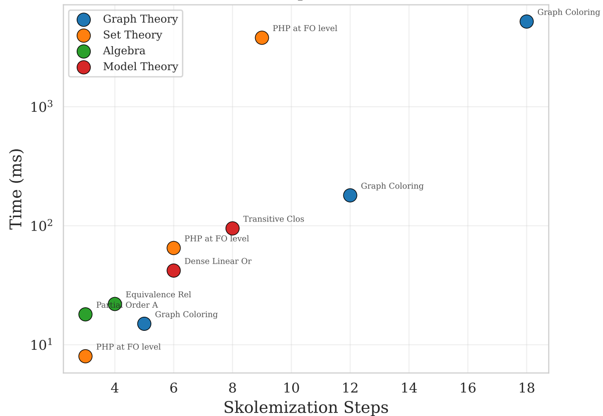
(b) Skolem Steps vs Solve Time
