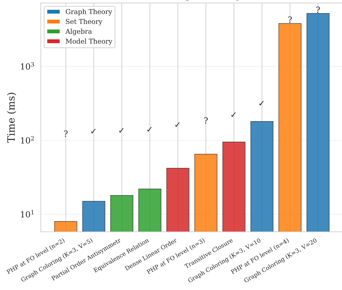
(a) FO Reasoning: Time by Domain
