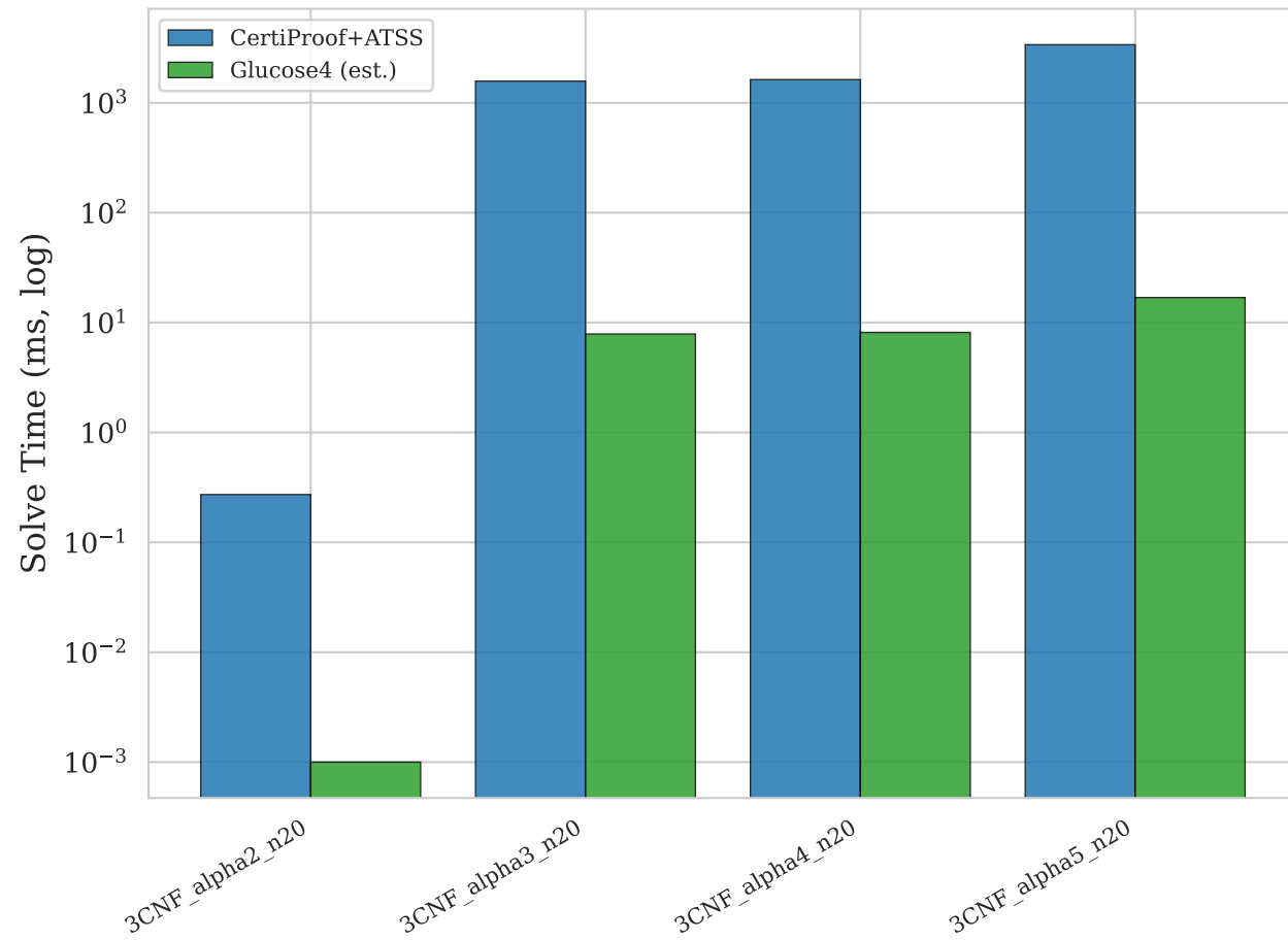
(a) SOTA Time Comparison
