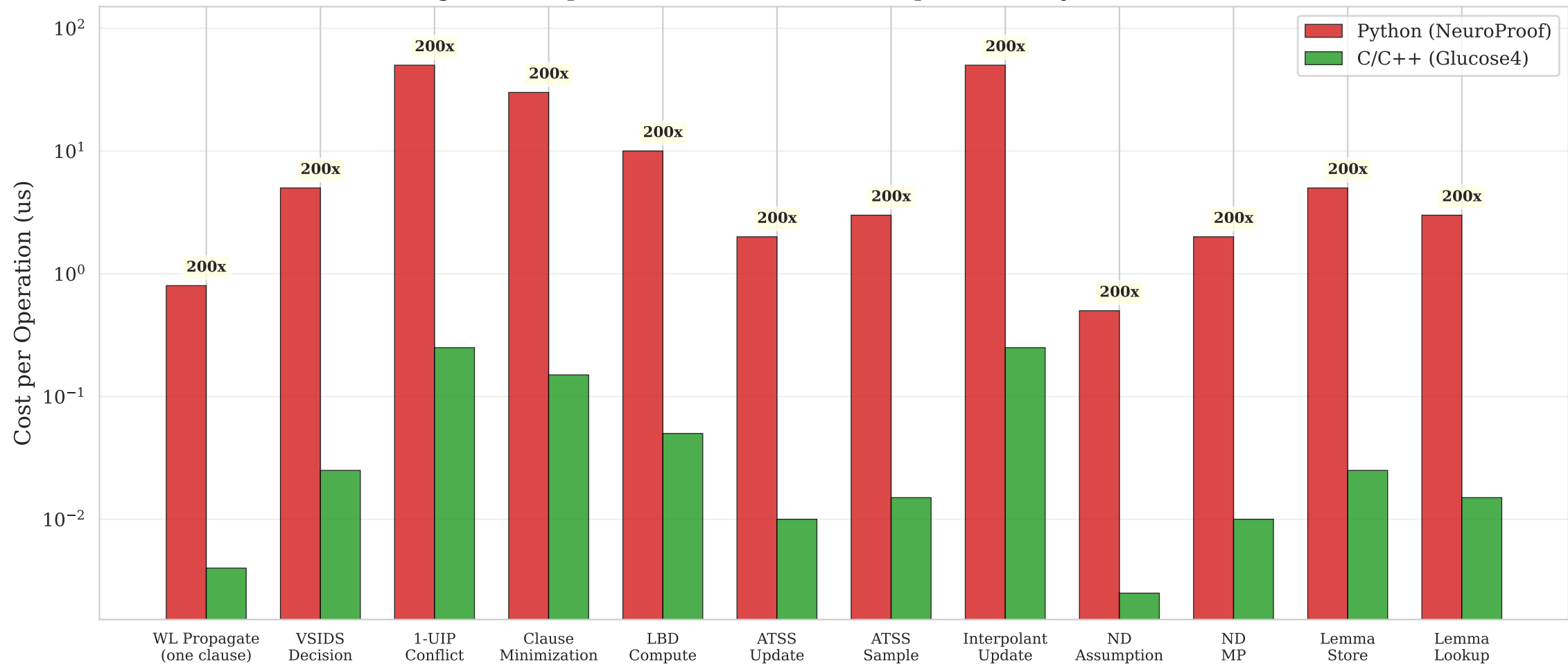
Figure 12: Operation Primitive Cost Comparison — Python vs C/C++
