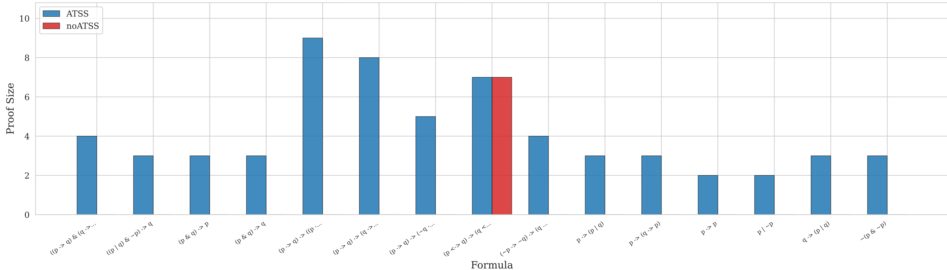
Fig 1: Classical Tautology Proof Sizes (ATSS vs noATSS)
