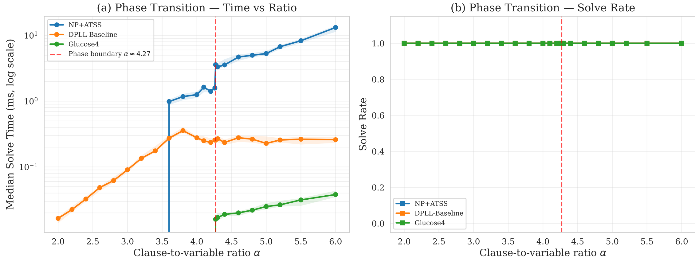
Figure 3: Phase Transition at n=20
