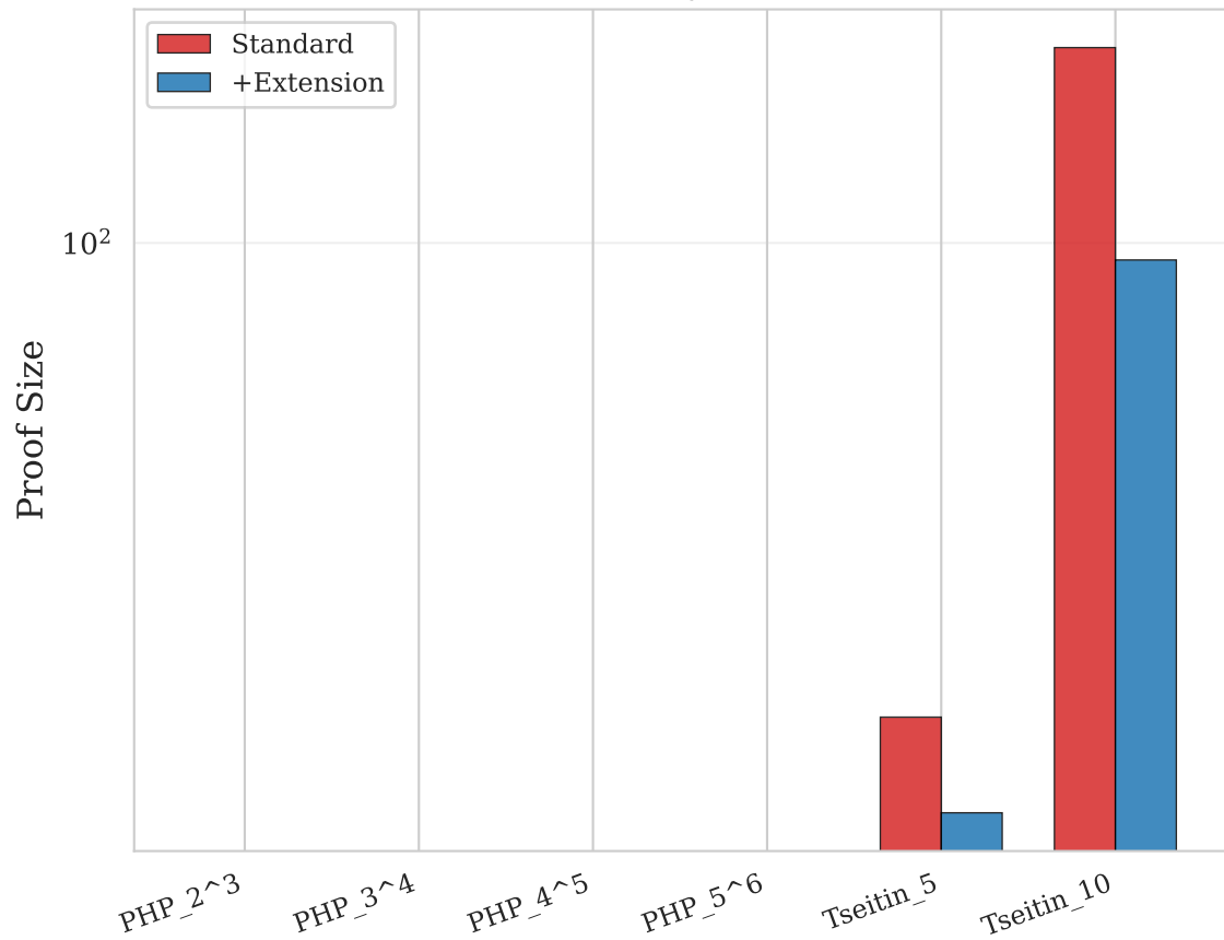
(b) Proof Size: Polynomial Speedup
