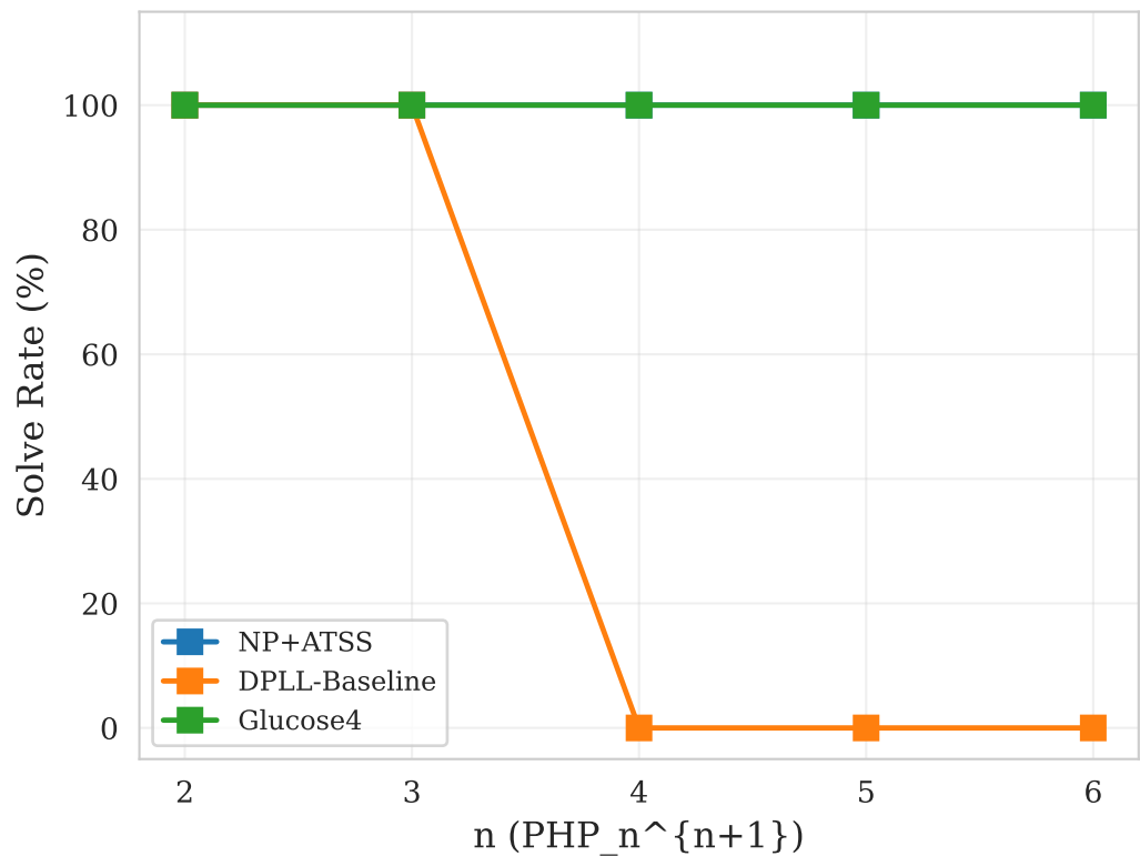
(b) PHP Solve Rate
