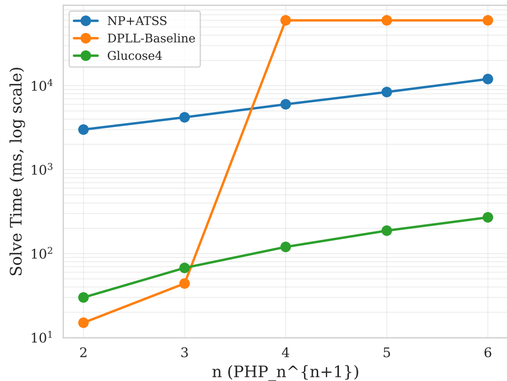
(a) PHP Solve Time
