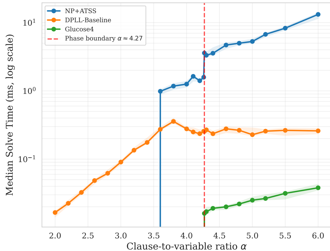
(a) Phase Transition — Time vs Ratio
