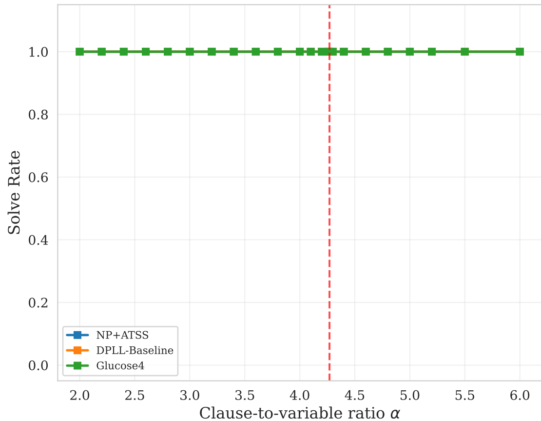
(b) Phase Transition — Solve Rate
