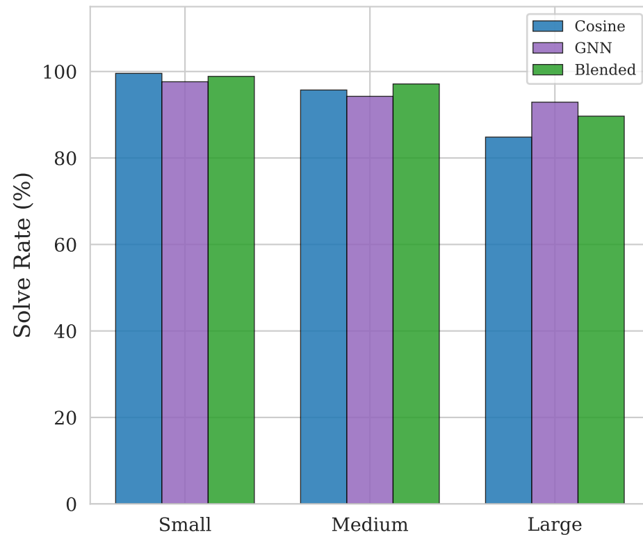
(b) Solve Rate
