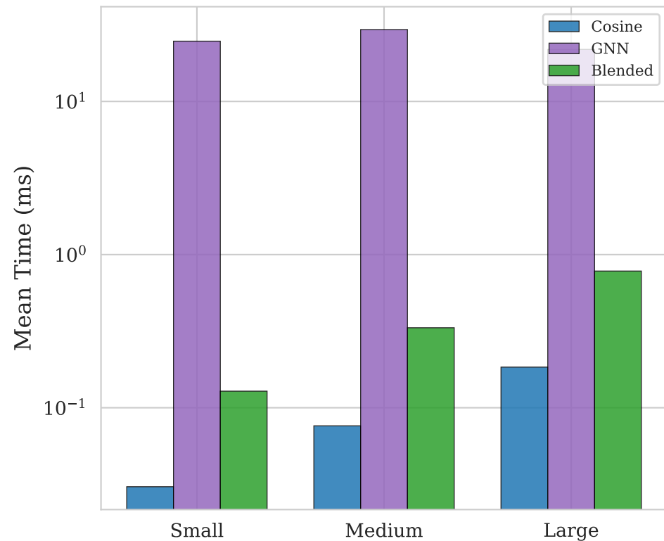
(a) Inference Time
