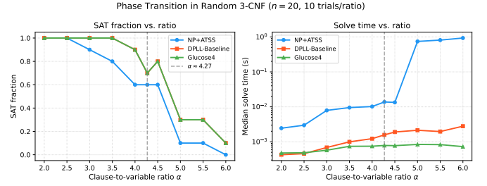
Fig. 2: Phase transition in random 3-CNF ( n = 20 , 10 trials per ratio). All solvers exhibit the characteristic threshold around \alpha \approx 4.27 . Glucose4 dominates on UNSAT instances; NEUROPROOF+ATSS performs comparably on SAT instances.
