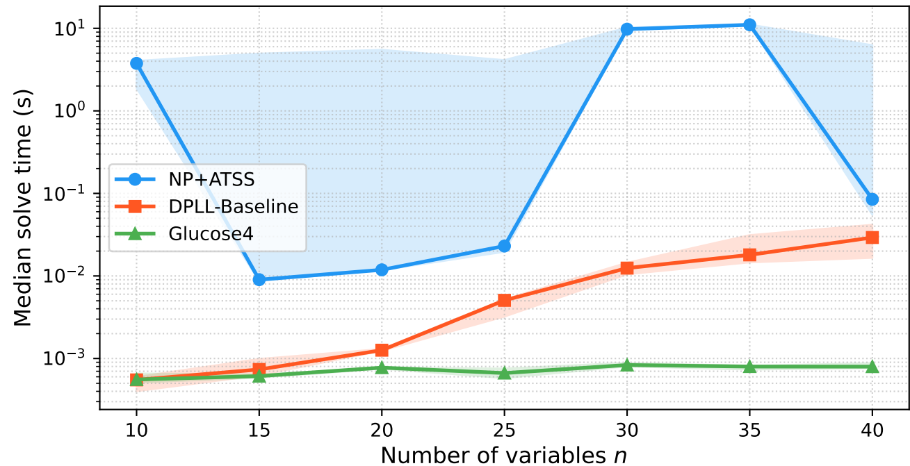
Scalability: solve time vs. n_{\text{vars}} ( \alpha = 4.27 , 3 trials/point)
