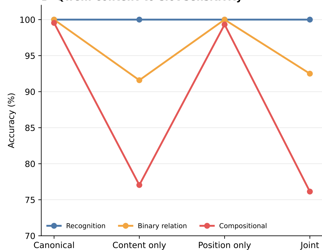
D Held-out controlled-natural test
