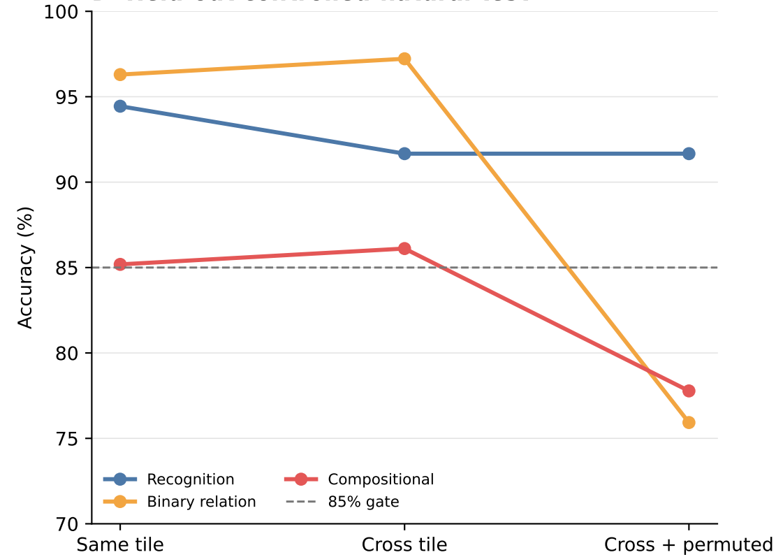
D Held-out controlled-natural test
