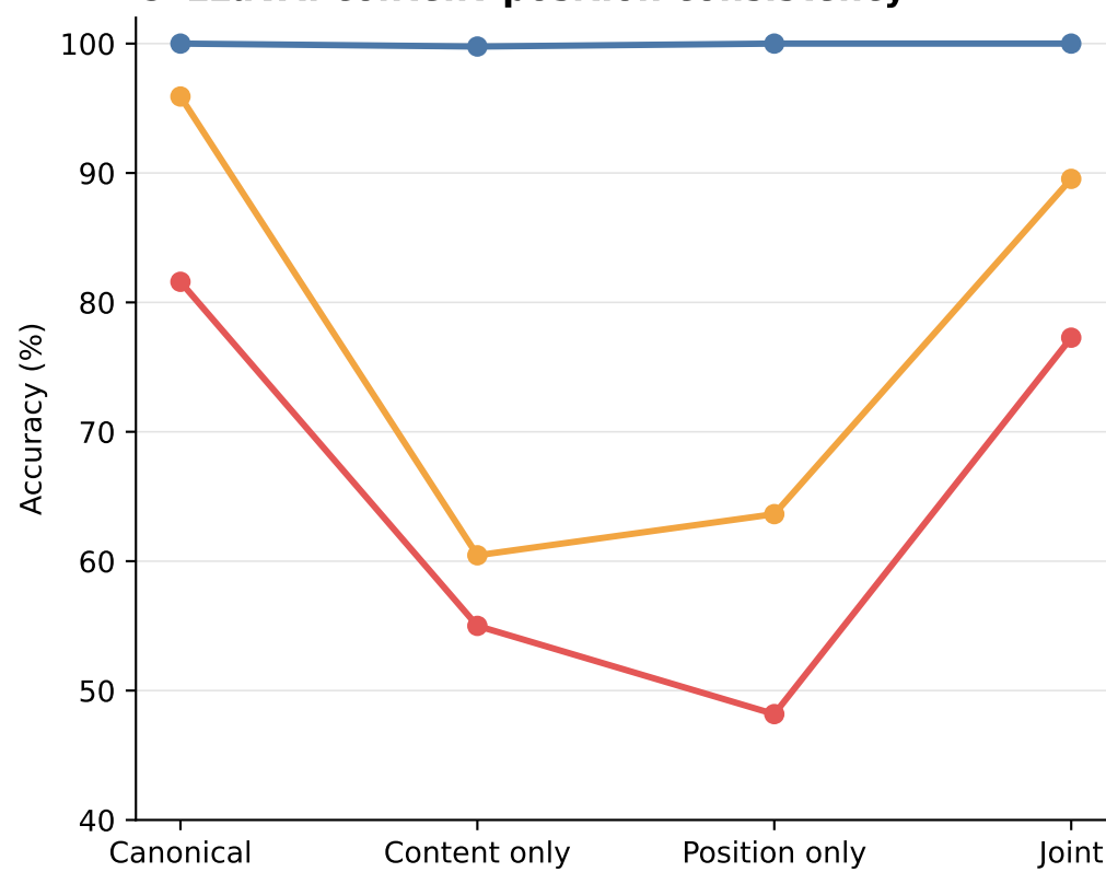
C LLaVA: content-position consistency
