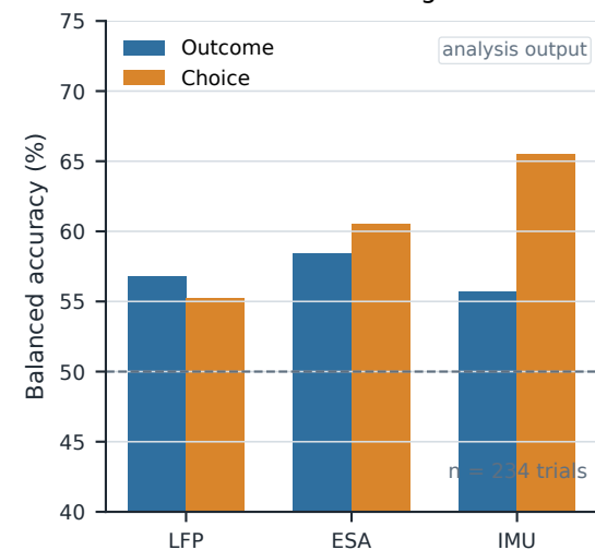
c Cross-validated decoding from trial-start window
