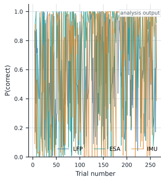
e Decoding confidence across trials
