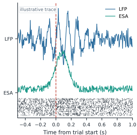
b Trial-aligned LFP, ESA and raster
