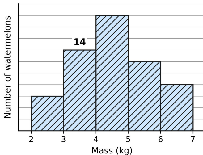
Masses of 60 watermelons
