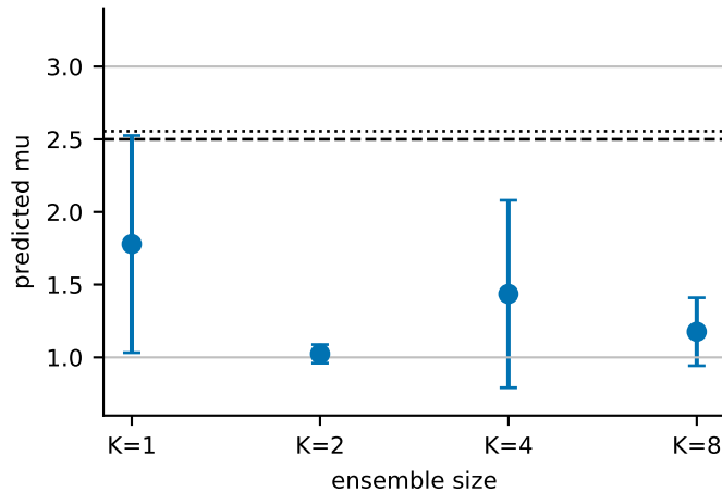
MLP ensemble, true mu = 2.5
