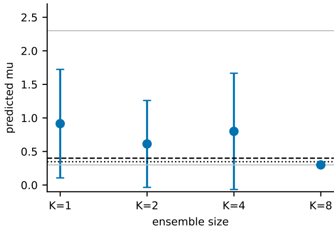
MLP ensemble, true mu = 0.4
