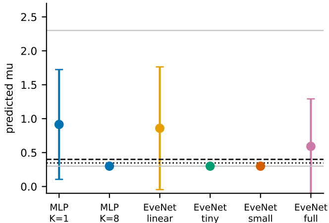
MLP vs EveNet heads, true mu = 0.4
