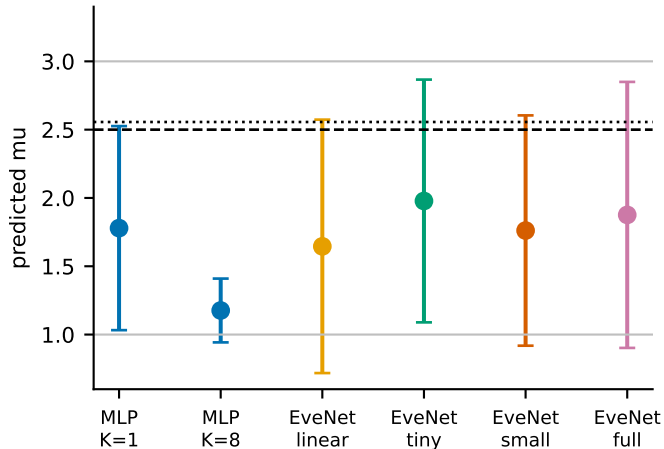
MLP vs EveNet heads, true mu = 2.5
