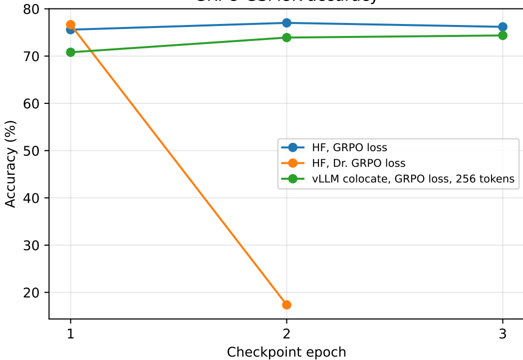
GRPO GSM8K accuracy
