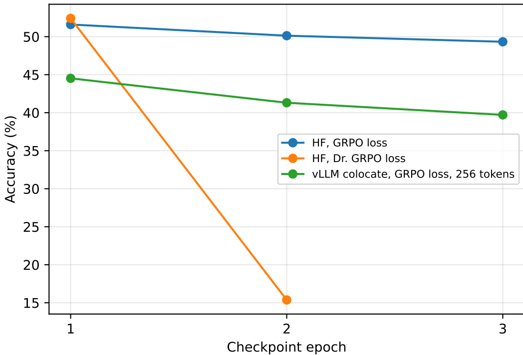
GRPO MMLU accuracy
