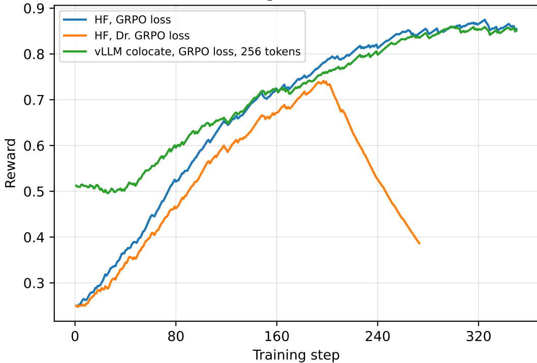
GRPO training reward (EMA 0.99)
