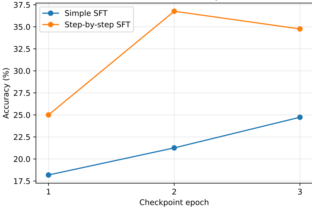
SFT MMLU accuracy
